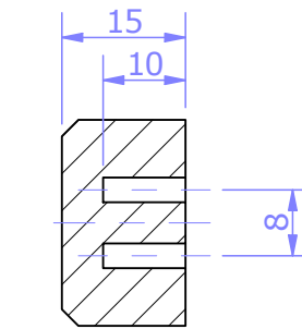
Section G-G
