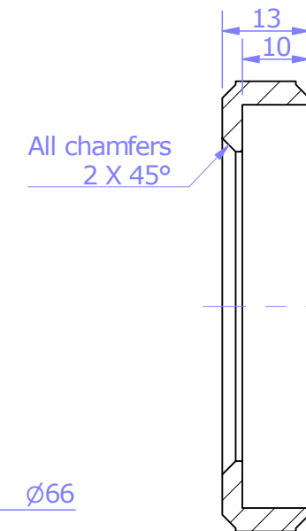
Section E-E
