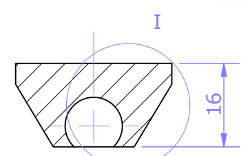
Section H-H
