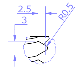
Detail F
