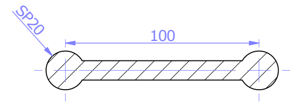
Section J-J
