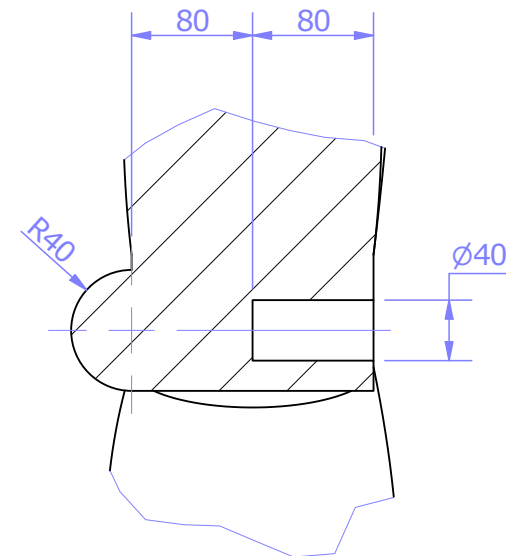
Detail E
