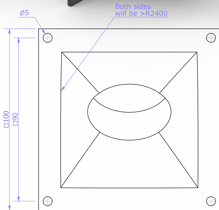
Elevation (Front)
