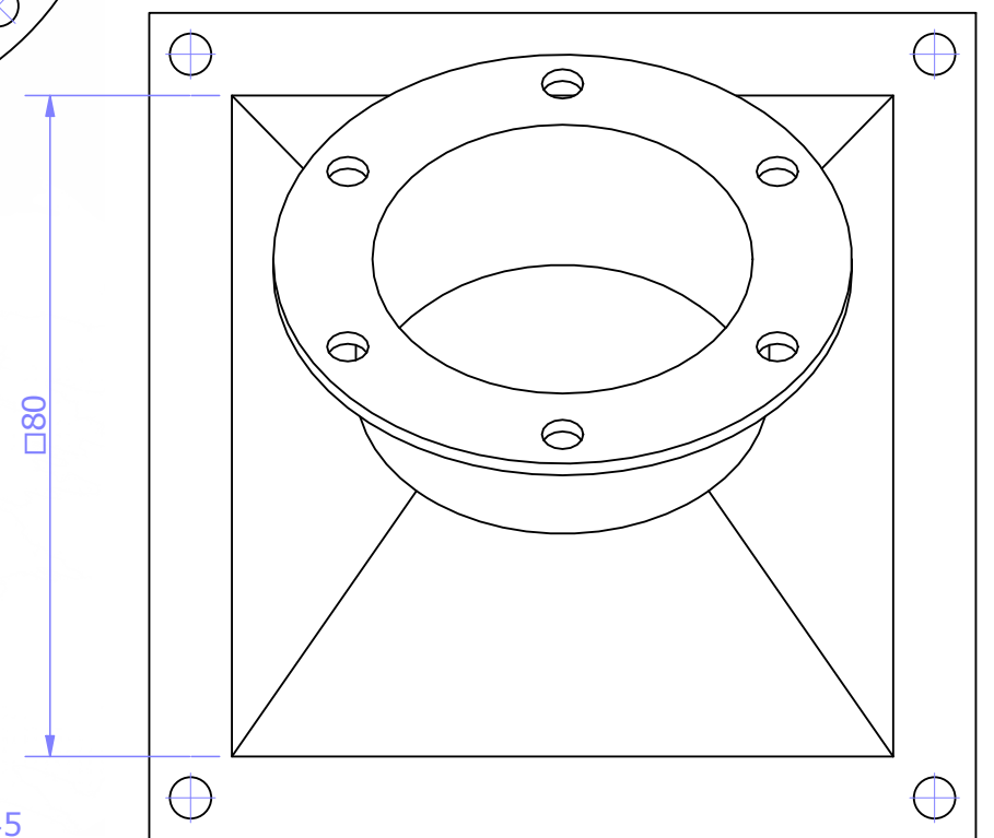
Elevation (Rear)
