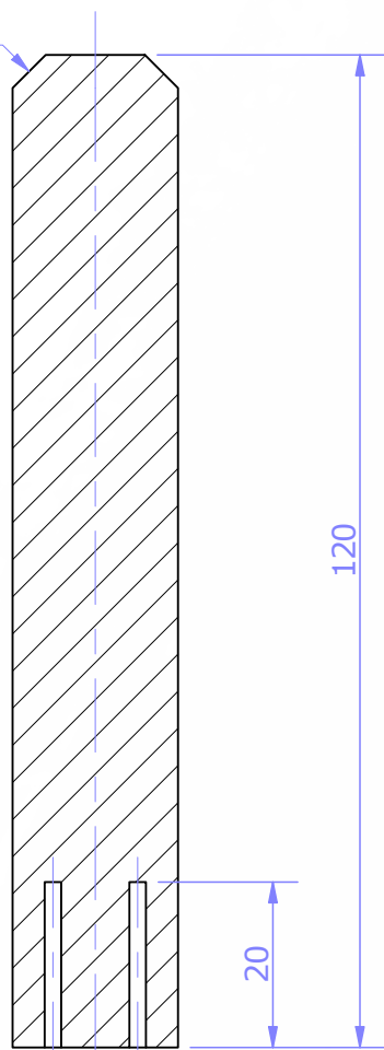
Section B-B
